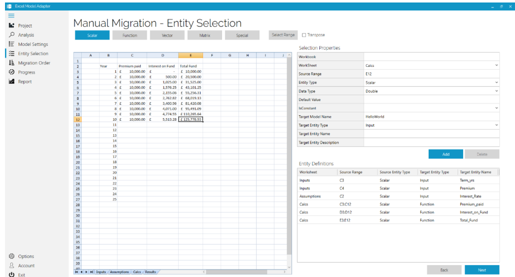
Figure 7 - Using EMA function to convert a spreadsheet model to Mo.net interactively
